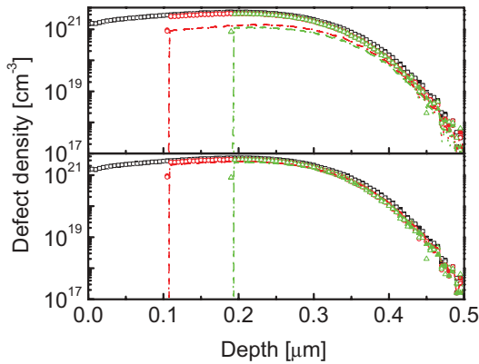
FIG. 5. (Color online) Postanneal total interstitial (filled symbols) and vacancy (empty symbols) defect densities for 2.6 [red (dark gray)] and 3.0 [green (light gray)] \text{J}/\text{cm}^2 laser fluences. Dark squares refer to the simulated total interstitial and vacancy defects after KMC room temperature evolution. Dashed ( I ) and dotted ( V ) lines refer to the continuous simulation carried out by means of the Giles et al. (upper panel) and Rafferty et al. (lower panel) parameters for cluster dissolution rates.
